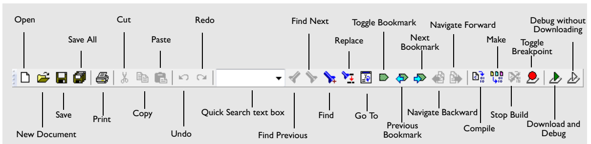
Figure 51: IDE toolbar
