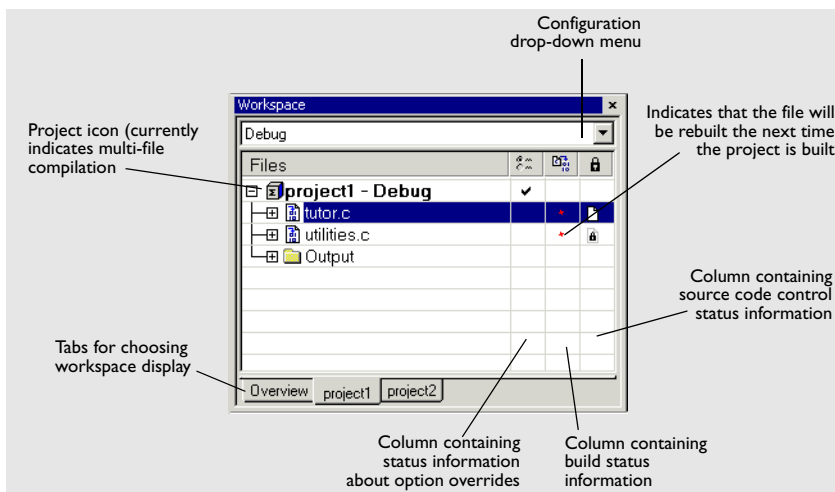
Figure 8: Workspace window
