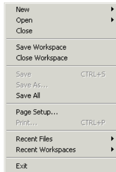
Figure 59: File menu
