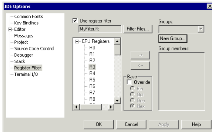
Figure 83: Register Filter options
