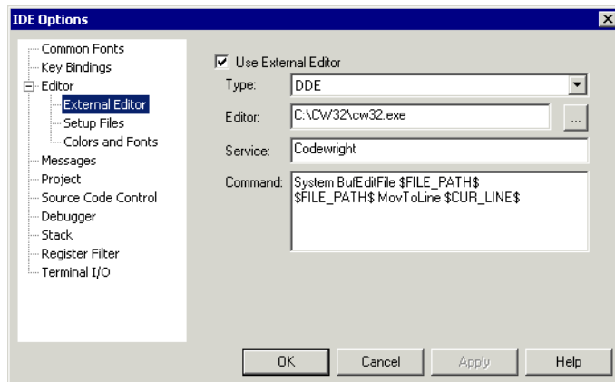
Figure 74: External Editor options
