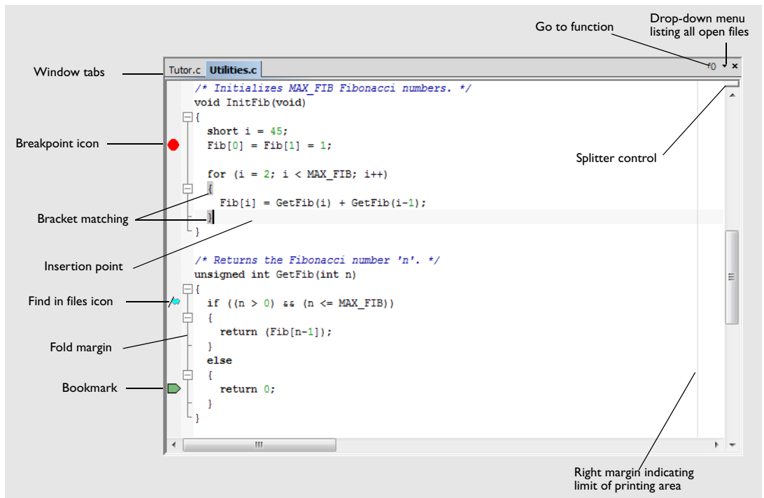
Figure 35: Editor window
