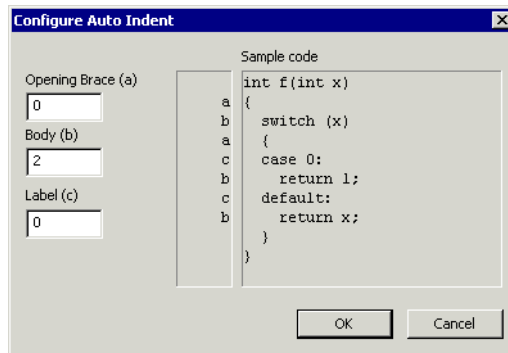
Figure 73: Configure Auto Indent dialog box
