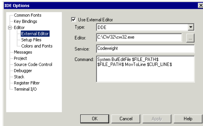
Figure 34: External editor DDE settings
