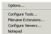
Figure 68: Tools menu
