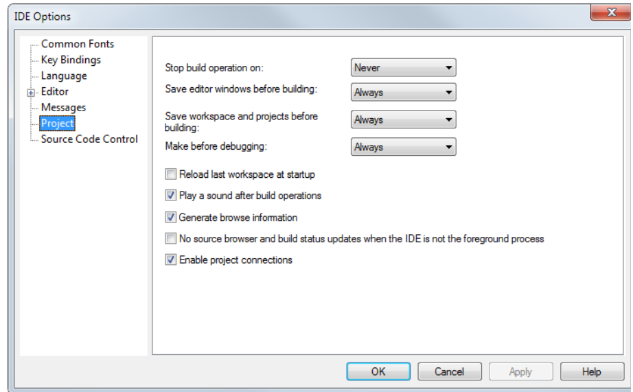
Figure 79: Project options
