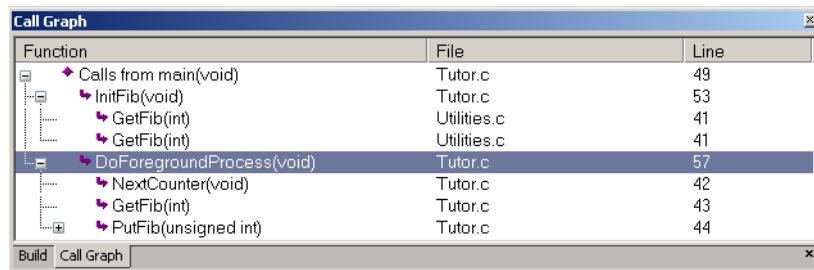
Figure 15: Call Graph window (calls from)
